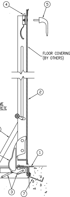
VIEW A ENLARGED SECTION OF NEOPRENE CUSHION & TILE EDGING
